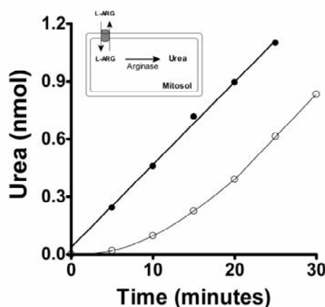
Figure 4 - Time course of L-arginine transport. Samples of N. neglecta liver mitochondrial fraction (-○-○-) and extracts (●-●-) were incubated in compartmentalization buffer without EDTA, pH 7.4, containing L-arginine 100mmol/l and MnCl_2 5mmol/l. The reactions were carried out at a temperature of 0°C near fish physiological conditions.
