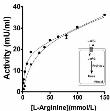
Figure 3 - Kinetic parameters involving the effect of L-arginine on the argininolytic activity. Aliquot of N. neglecta liver mitochondrial extracts (-●-) and suspension (-▲-) were incubated in compartmentalization buffer without EDTA, pH 7.4 containing MnCl_2 0.5mmol/l. The reactions were carried out at a temperature of 0°C.
